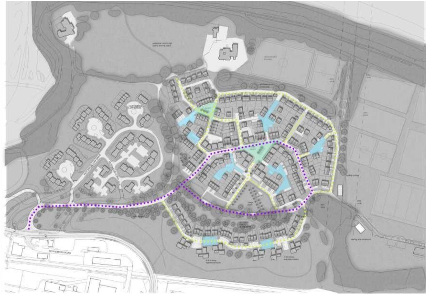
FIG 78: STREET HIERARCHY
