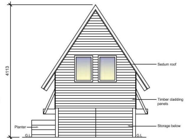
Proposed Rear Elevation (East)
