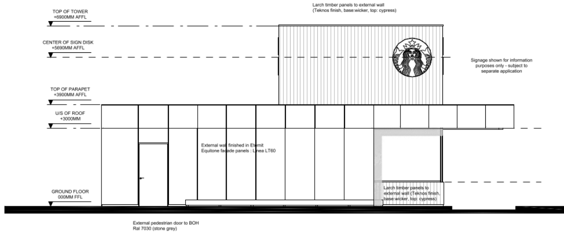
East Elevation
